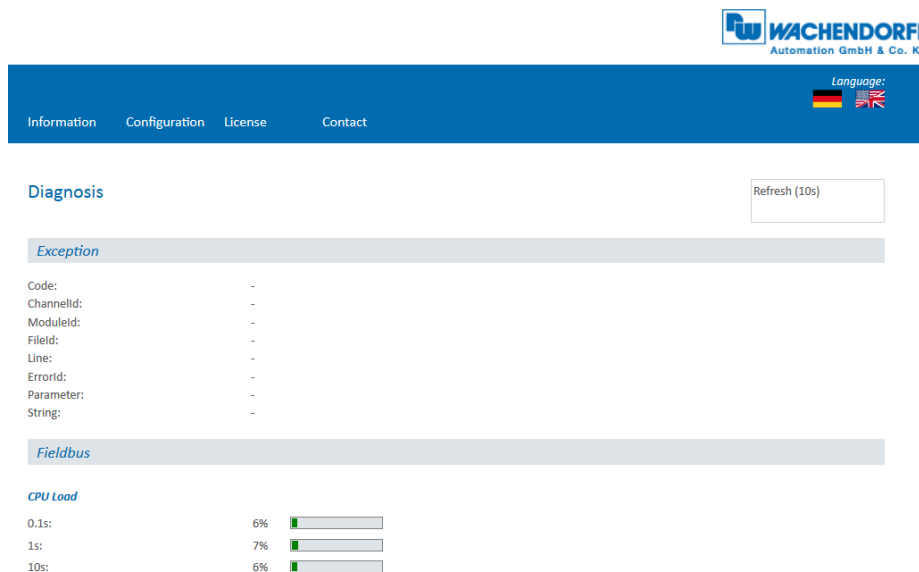
Figure 5.2: Diagnostics page
